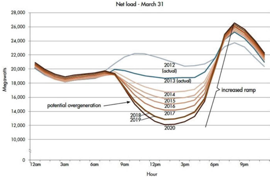
Fig. 1.6 The California ISO duck curve [4]
