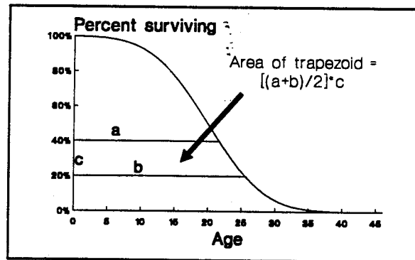
Figure 6-3. Calculation of Average Life from Survivor Curve.
