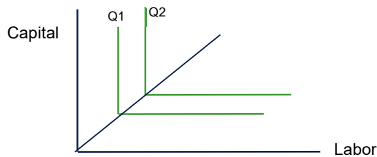
Figure B-1: Representation of a typical Leontief Isoquant Map
